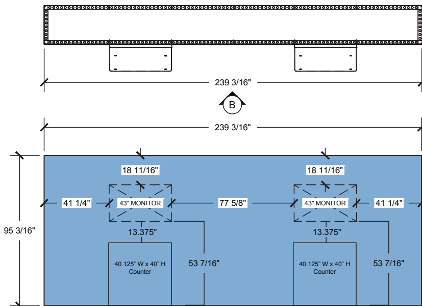
Elevation B (SEG/Fabric)
