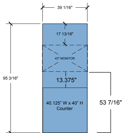
Elevation A (PVC)
