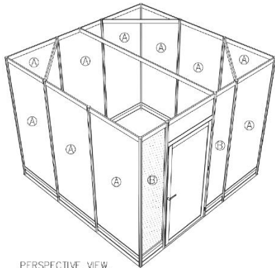
PERSPECTIVE VIEW
