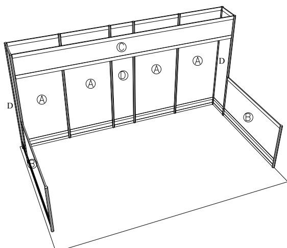
PERSPECTIVE VIEW
