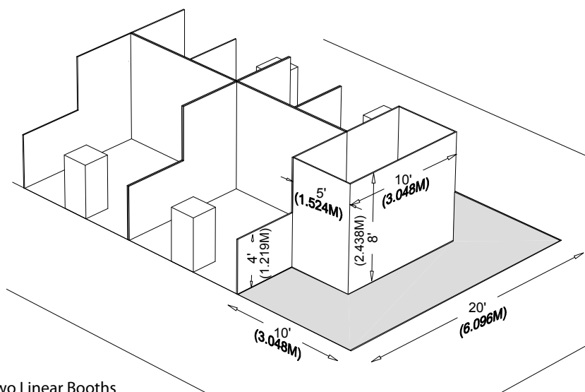
End-cap to two Linear Booths
