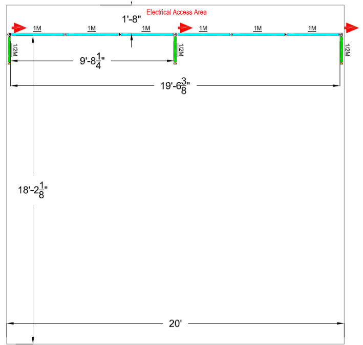
20x20 Actual Working Space Layout Backwalls Shared w/ Raw Spaces or Collective Booth Packages
