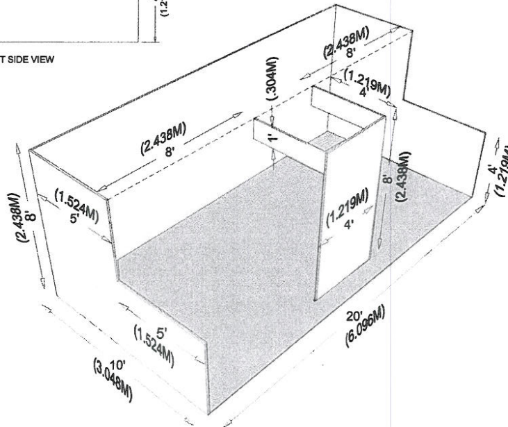
10' X 20' EXTENDED HEADER BOOTH
